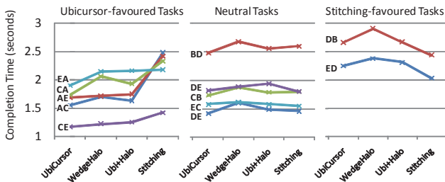
Figure 8. Performance profiles of each path (in seconds), split left to right into three kinds of tasks. Each line represents a task, labeled on its left with origin and destination display. To highlight the profiles, the scales start at 1 s.
